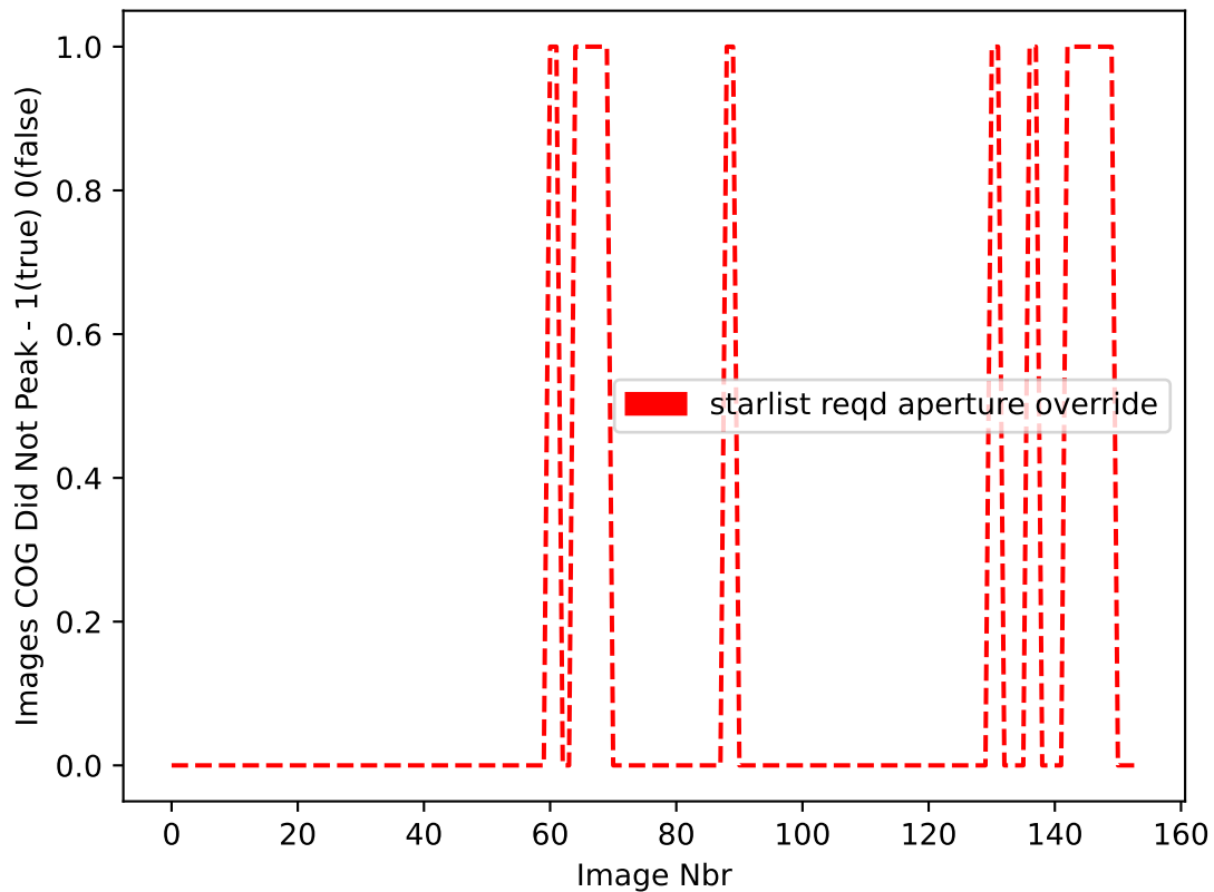
Images Where SNR COG Did Not Peak
