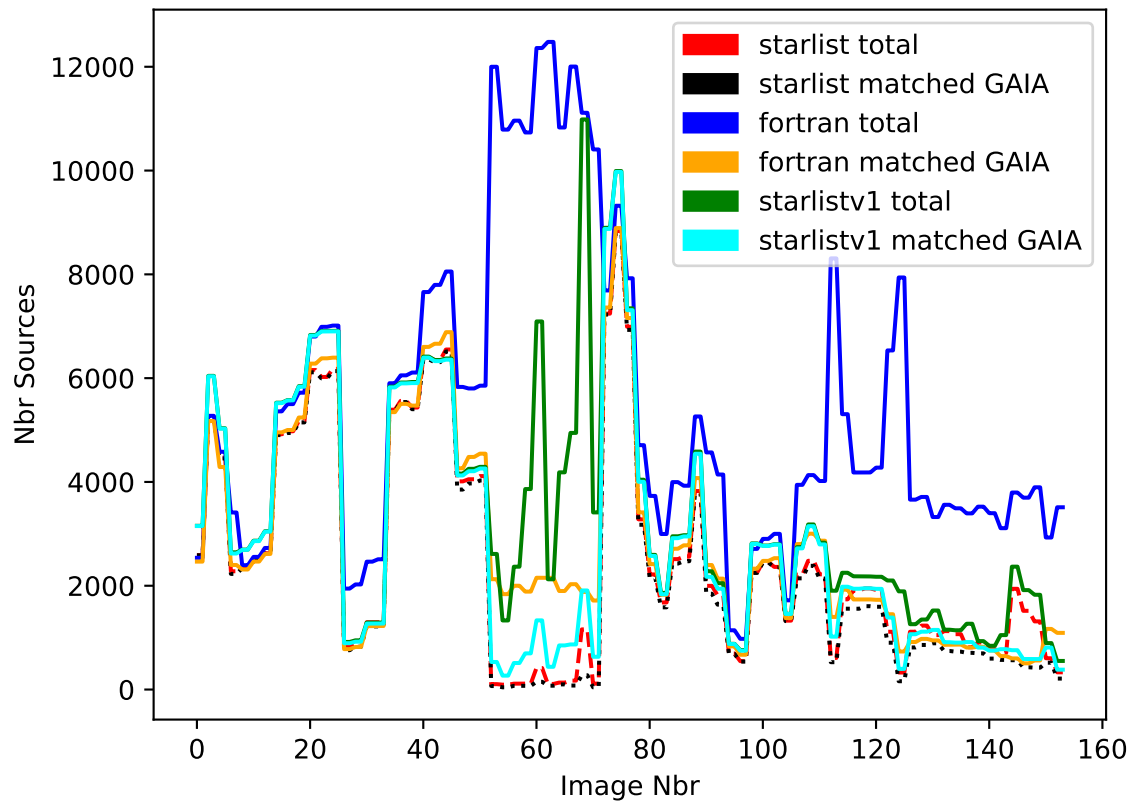
Number of Sources Total and Valid
