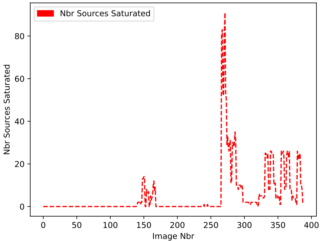
Saturated Sources
